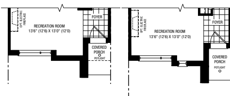
PARTIAL GROUND B PARTIAL GROUND C
