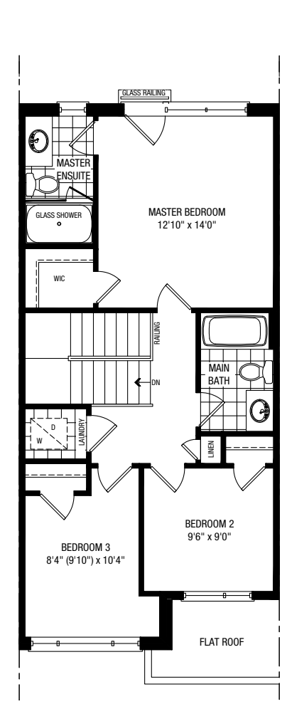
PARTIAL THIRD B
