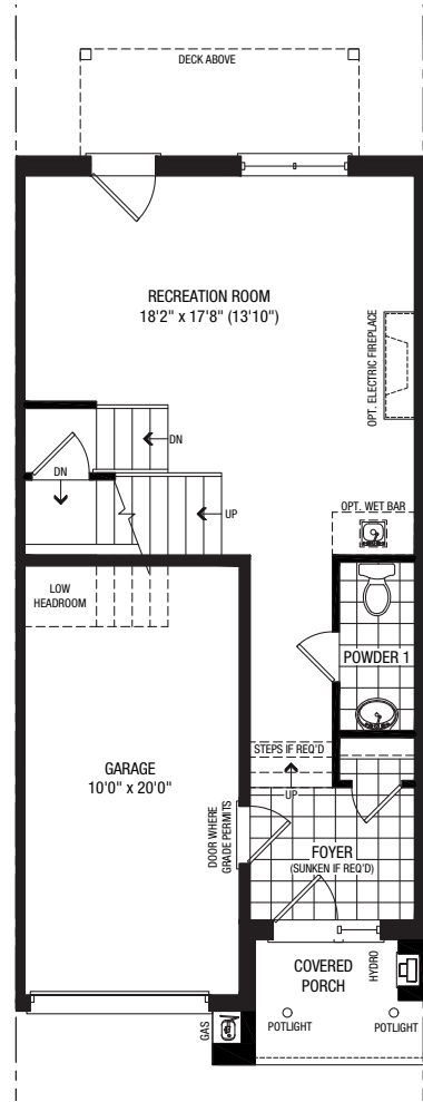
PARTIAL GROUND B
