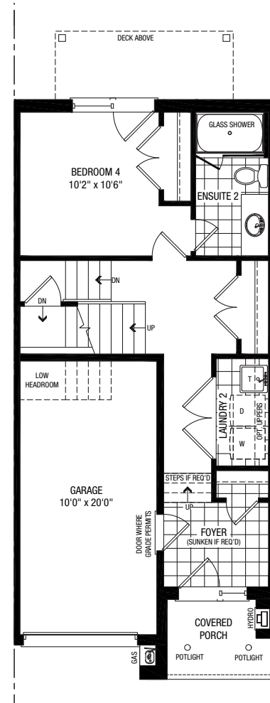
PARTIAL OPT. GROUND B
