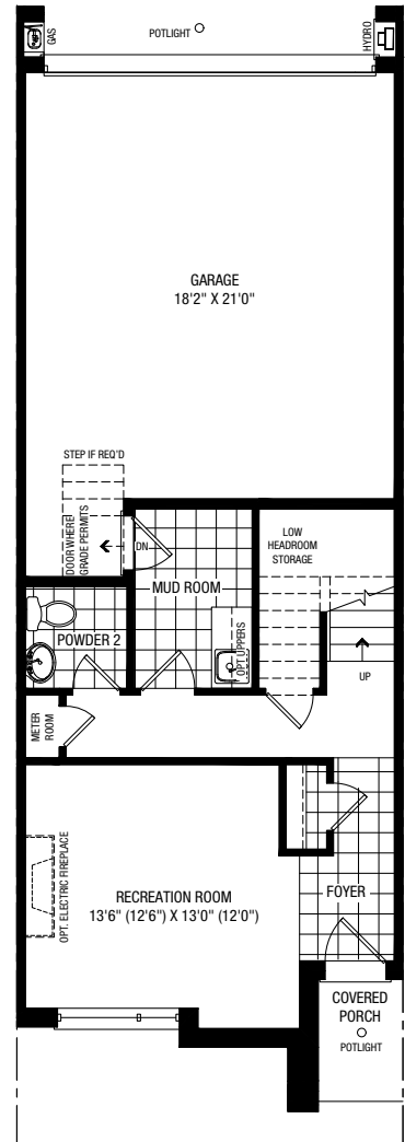
PARTIAL GROUND B PARTIAL GROUND C
