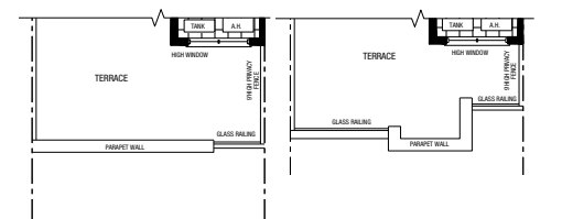
PARTIAL TERRACE B PARTIAL TERRACE C
