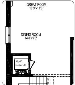
PART. GROUND FLOOR WITH OPT. ELEVATOR Elevation A
