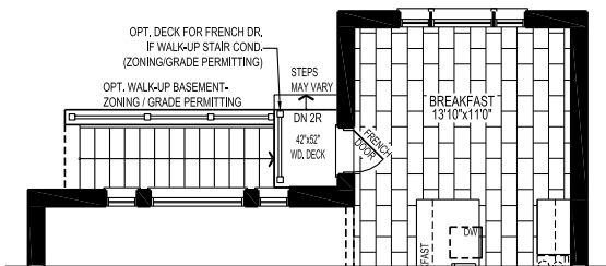
PART. GROUND FLOOR WITH OPT. DECK AND WALK-UP STAIR BASEMENT Elevation B
