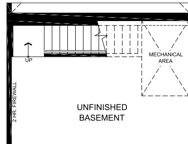
ELEVATION A1 PARTIAL BASEMENT W/O SUNKEN AREA
