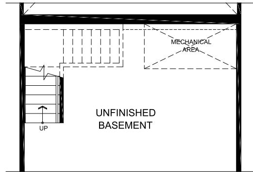
ELEVATION C1 PARTIAL BASEMENT W/O SUNKEN AREA
